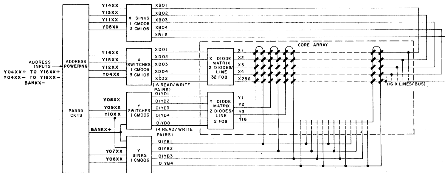
Figure 2-28. Address Decoding and Selection
