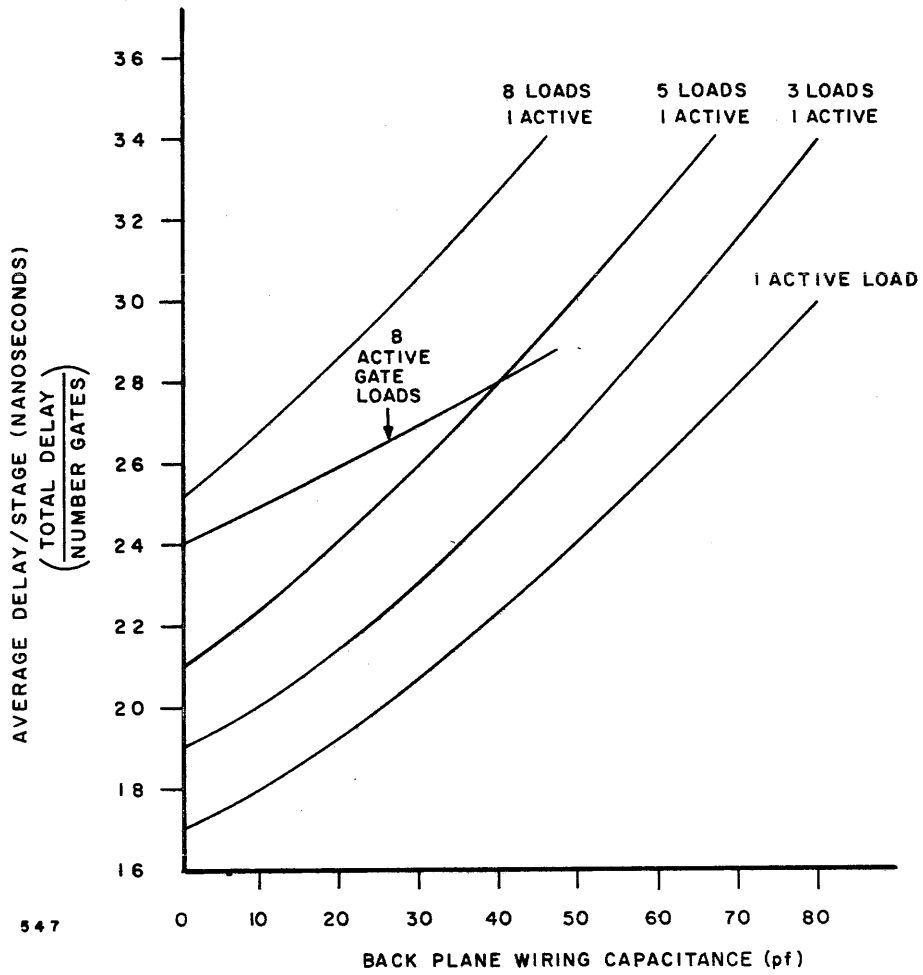
A-2. Typical NAND Gate Circuit Delays (Sheet 2 of 3)
