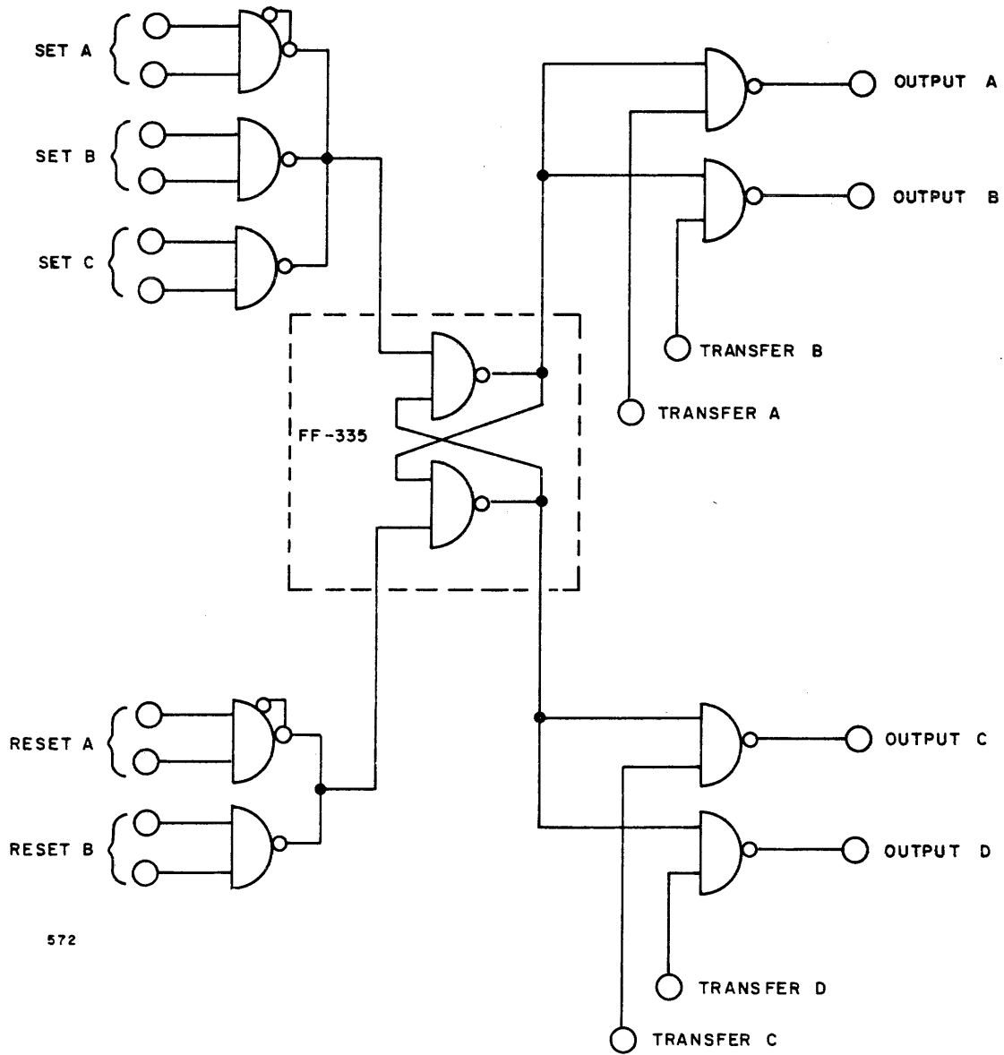
Figure A-92. Basic Flip-Flop PAC, Model FF-335, Input and Output Logic
