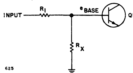
Figure A-108. Schmitt Trigger PAC, Model ST-335, Shifting Input Signal Network
