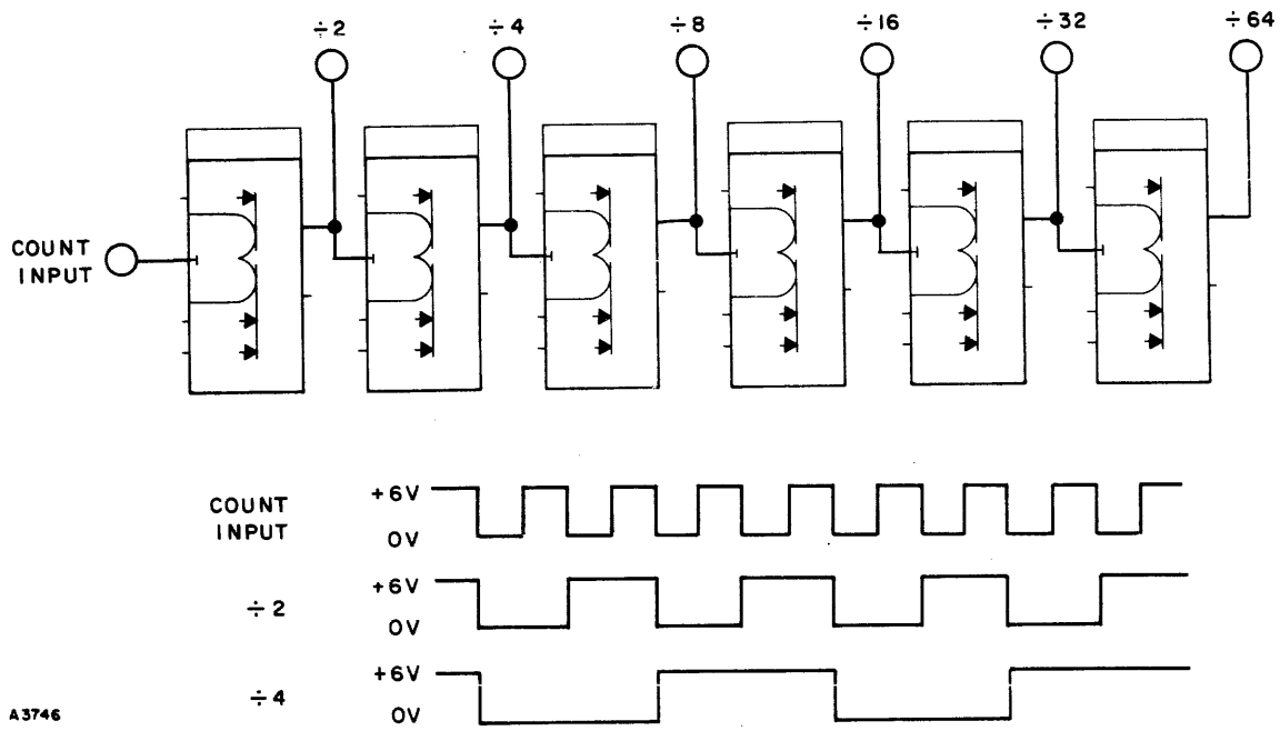
Figure A-49. Counter PAC, Model CC-088, Operation As a Frequency Divider
