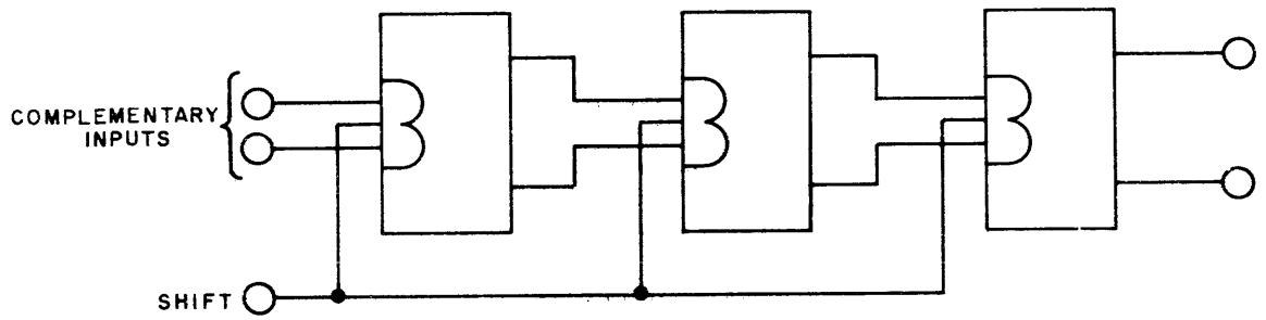
Figure A-53. Gated Flip-Flop PAC, Model CC-089, Shift Register Operation
