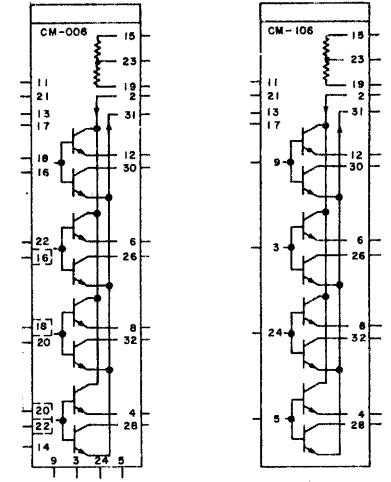
LOGIC SYMBOL
