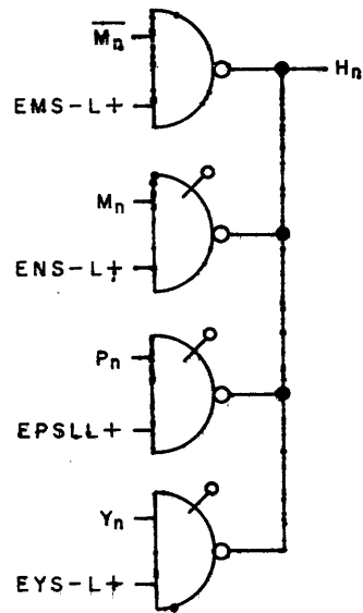
Figure 2-12. Summand Selection
