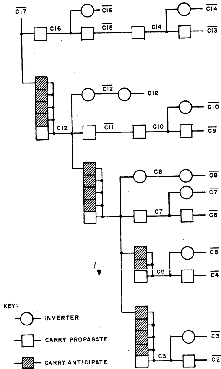
Figure 2-15. Carry Network Simplified Block Diagram
