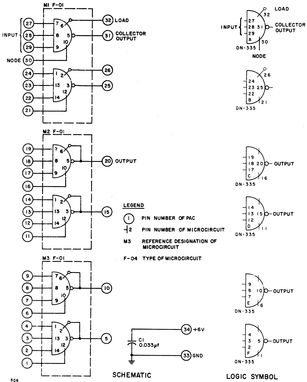
Figure A-86. Expandable NAND PAC, Model DN-335, Schematic Diagram and Logic Symbol
