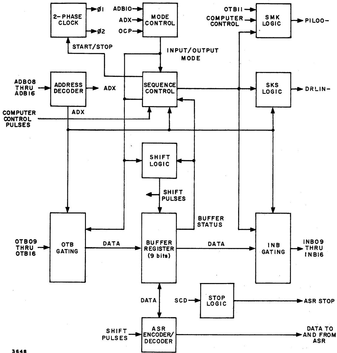
Figure 2-31. ASR Interface Block Diagram
