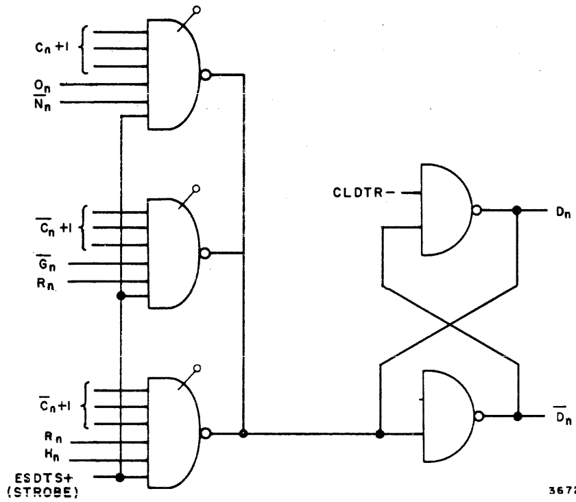
Figure 2-16. Sum Formation
