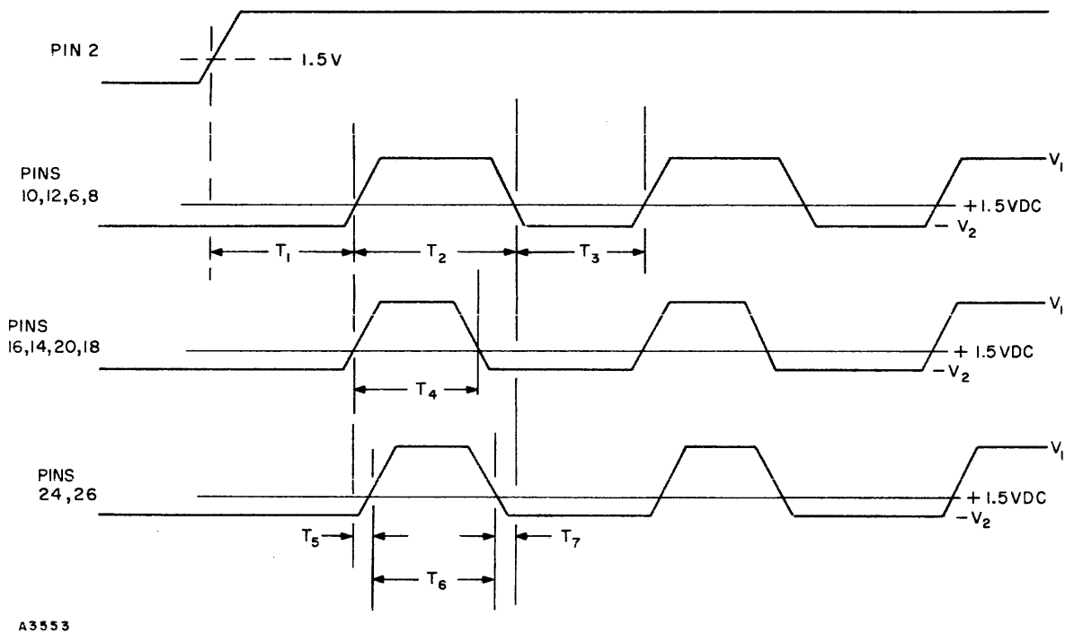
Figure A-29. Master Oscillator PAC, Model CC-046, Timing Diagram
