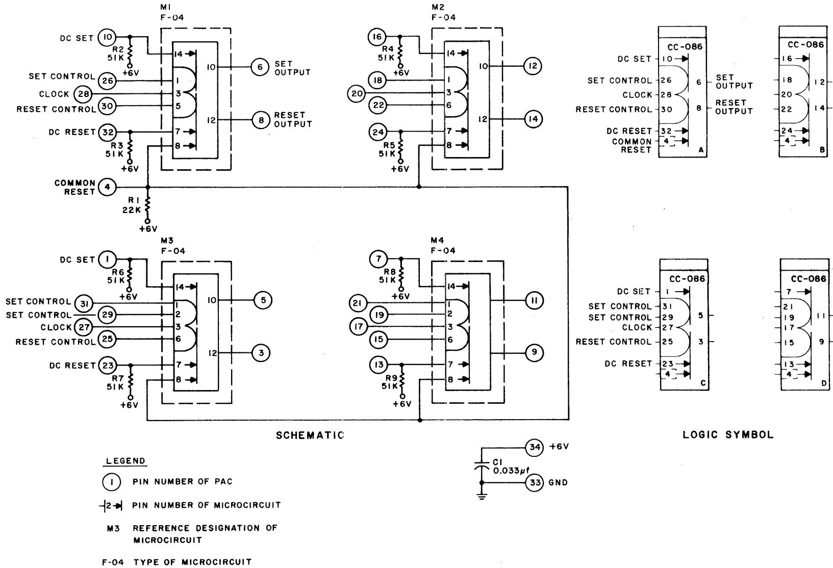
Figure A-42. Gated Flip-Flop PAC, Model CC-086, Schematic Diagram and Logic Symbol
