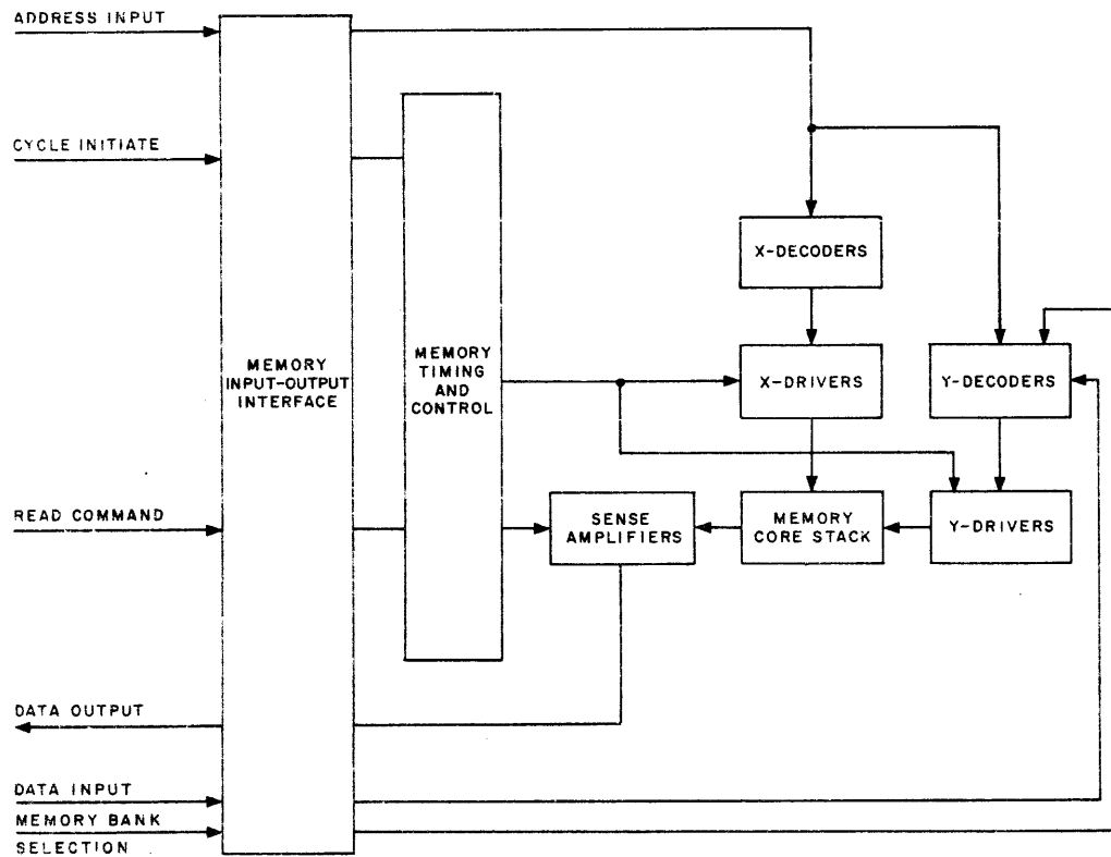
Figure 2-24. Memory Block Diagram
