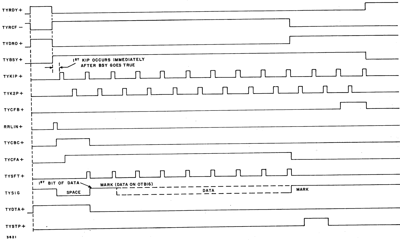
Figure 2-33. Output Mode Timing
