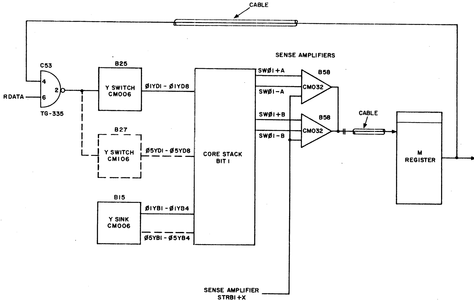
Figure 2-30. Regeneration Loop Simplified Diagram
