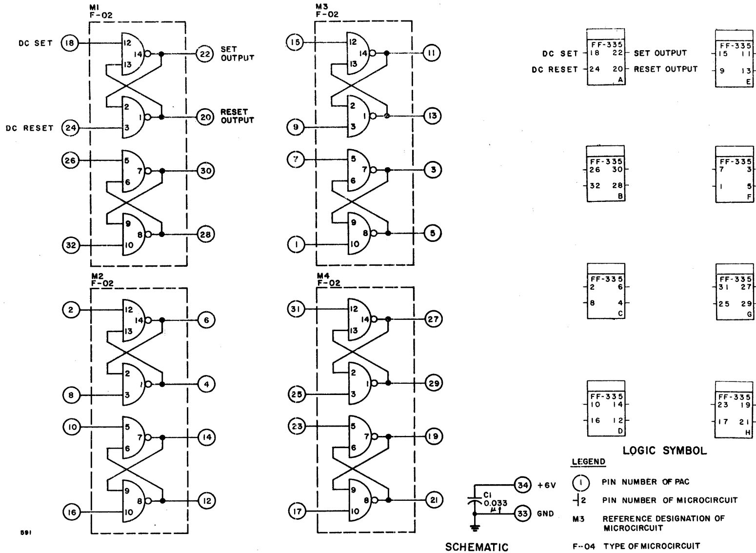
Figure A-89. Basic Flip-Flop PAC, Model FF-335, Schematic Diagram and Logic Symbol
