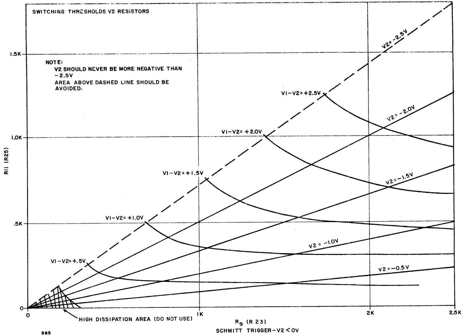
Figure A-107. Schmitt Trigger PAC, Model ST-335, Graph II
