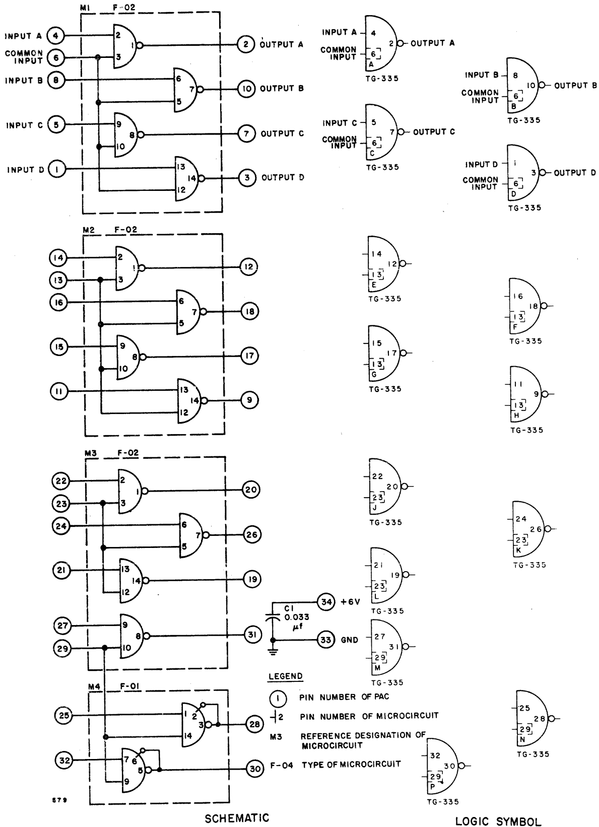
Figure A-109. Transfer Gate PAC, Model TG-335, Schematic Diagram and Logic Symbol
