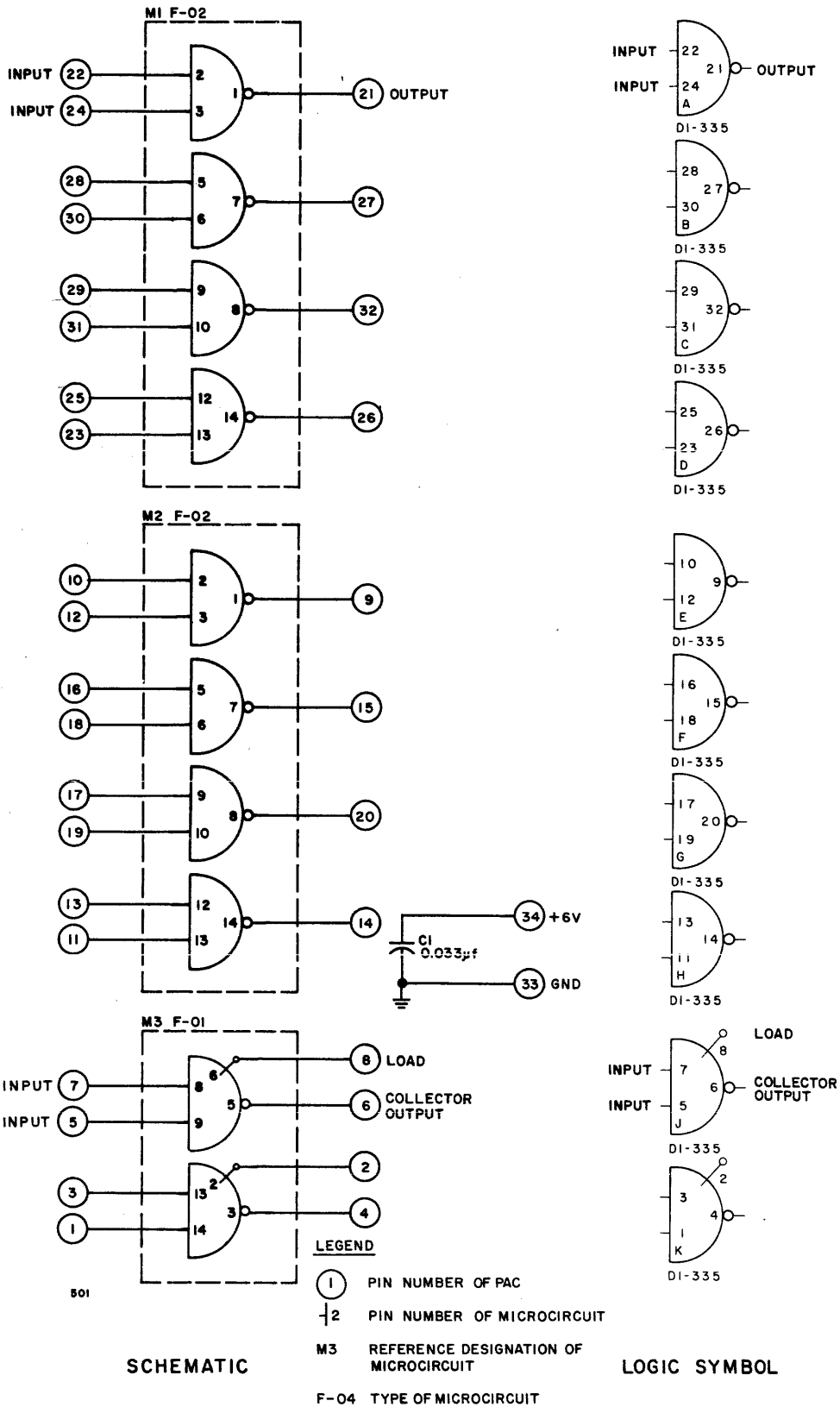
Figure A-76. NAND Type I PAC, Model DI-335, Schematic Diagram and Logic Symbol
