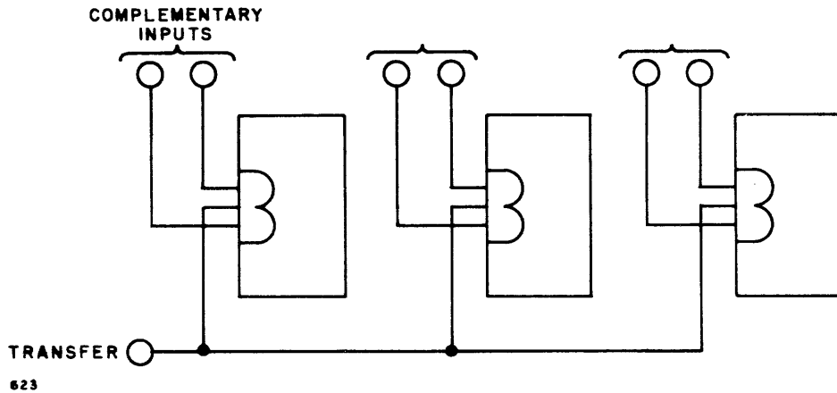
Figure A-41. Universal Flip-Flop PAC, Model CC-085, Parallel Information Drop-In
