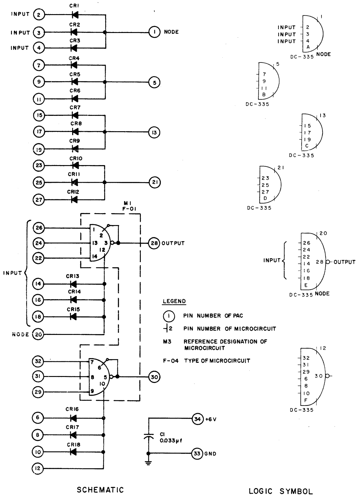
Figure A-73. Multi-Input NAND PAC, Model DC-335, Schematic Diagram and Logic Symbol
