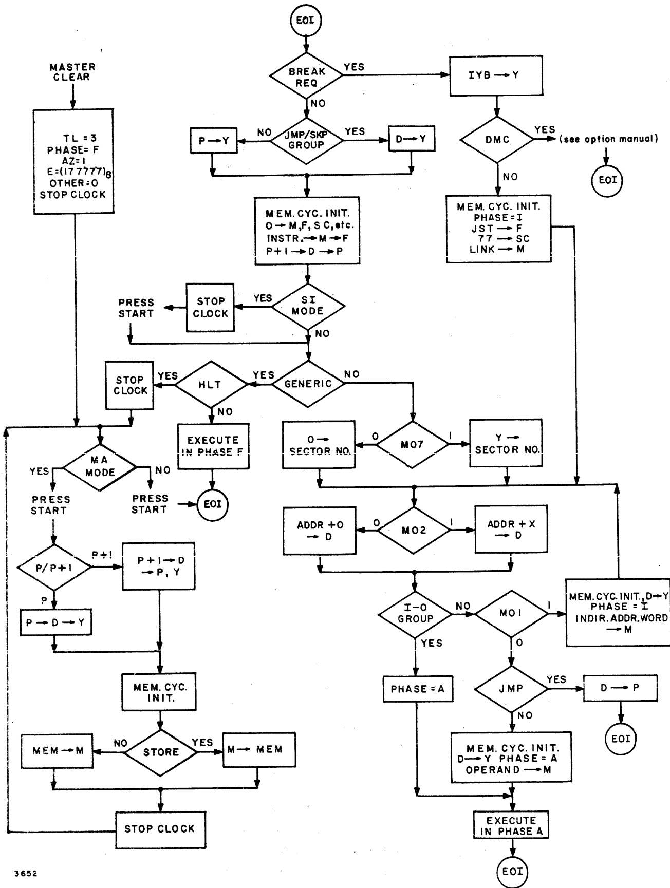
Figure 2-9. Basic Control Flow Chart
