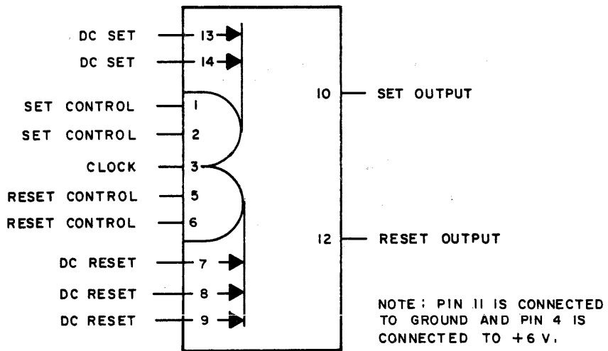
A. LOGIC SYMBOL
