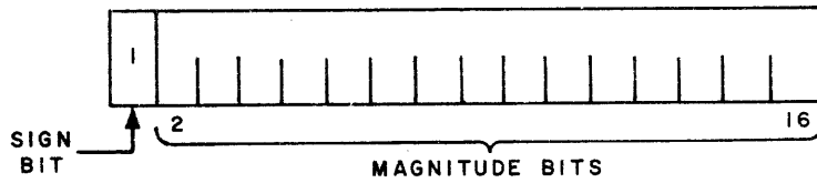
Figure 2-1. Data Word Format, Single-Precision
