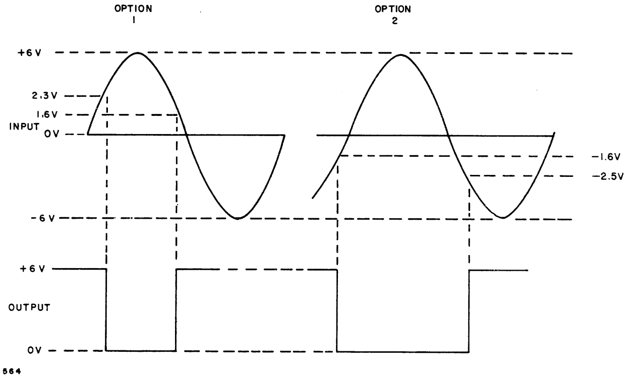
Figure A-105. Schmitt Trigger PAC, Model ST-335, Typical Waveforms
