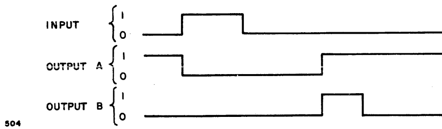
504 Figure A-85. Delay Multivibrator PAC, Model DM-335, Delayed Pulse Generator
