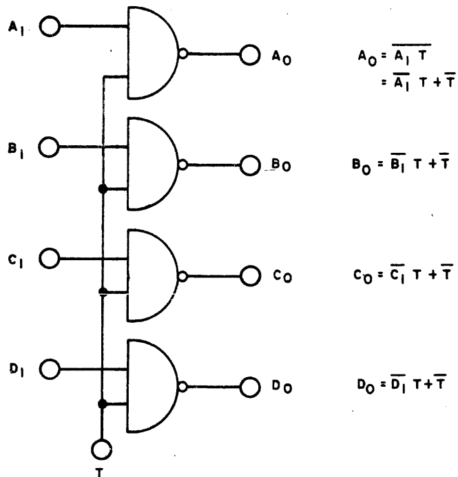
Figure A-111. Transfer Gate PAC, Model TG-335, Gate Structure Logic
