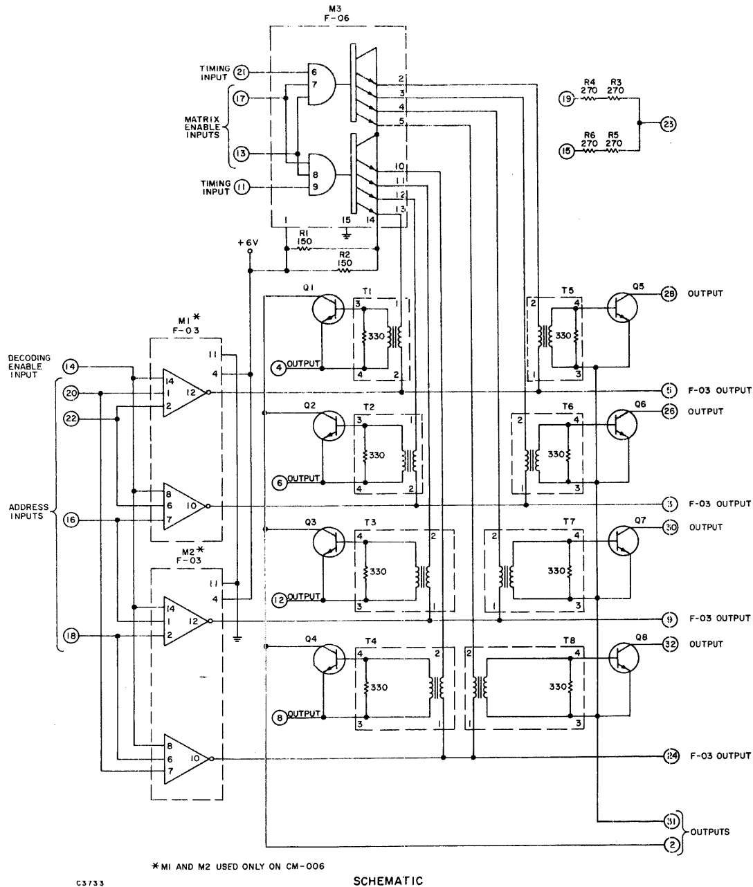
SCHMATIC
