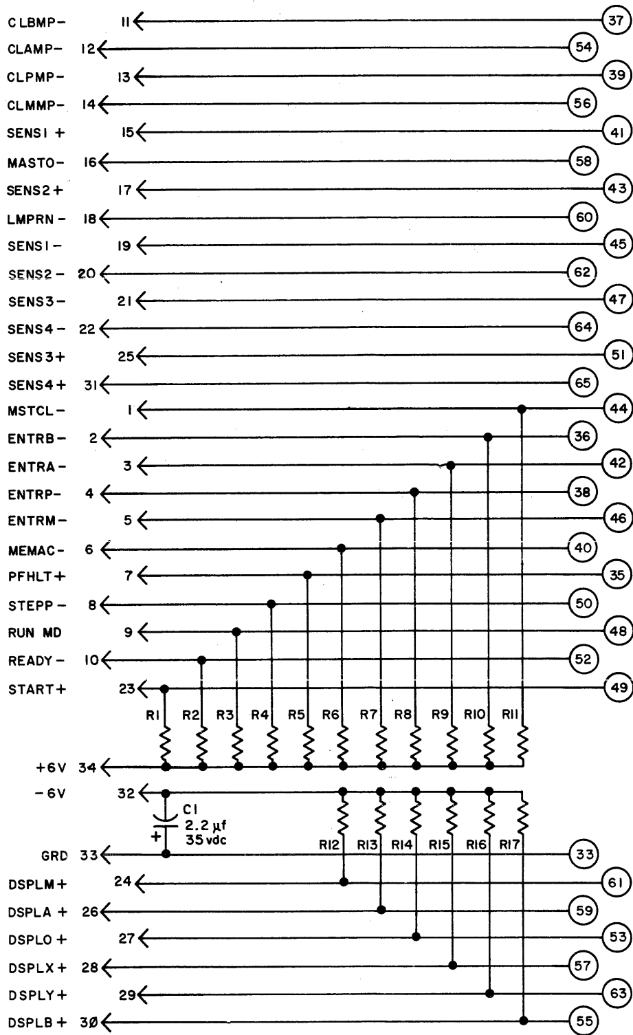
Figure A-35. Cable PAC, Model CC-080, Schematic Diagram
