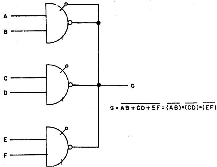
Figure A-88. Gates Used in Parallel
