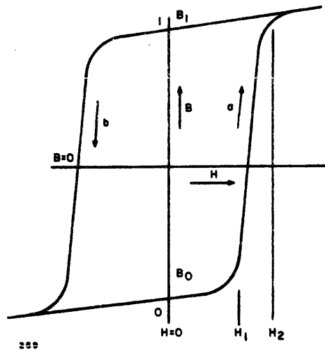
Figure 2-26. Typical B-H Characteristics
