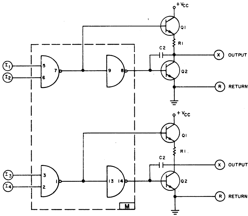
TYPICAL CIRCUIT
