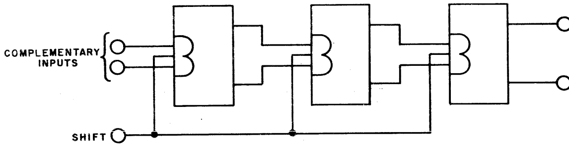
Figure A-62. Buffer Register PAC, Model CC-092, Shift Register Operation
