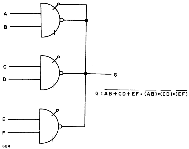
Figure A-78. NAND Type 1 PAC, Model DI-335, Gates Used in Parallel
