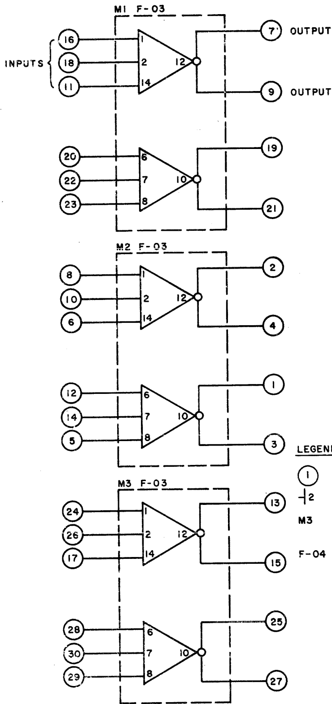
SCHMATIC
