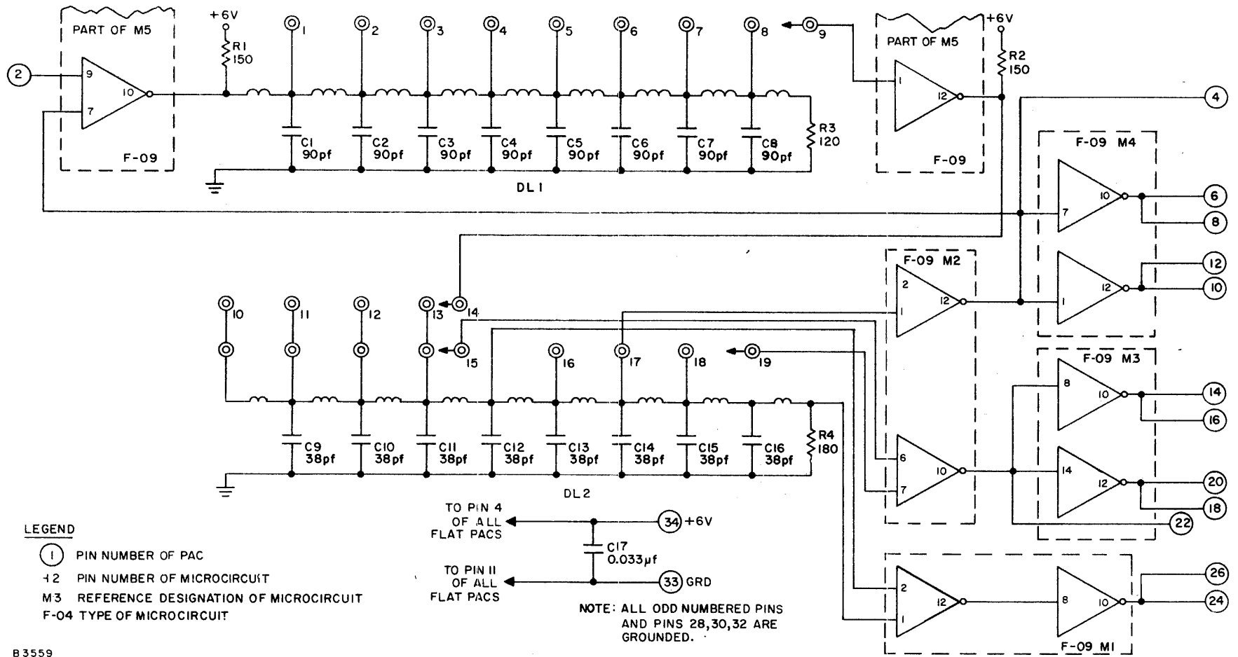
Figure A-30. Master Oscillator PAC, Model CC-046, Schematic Diagram
