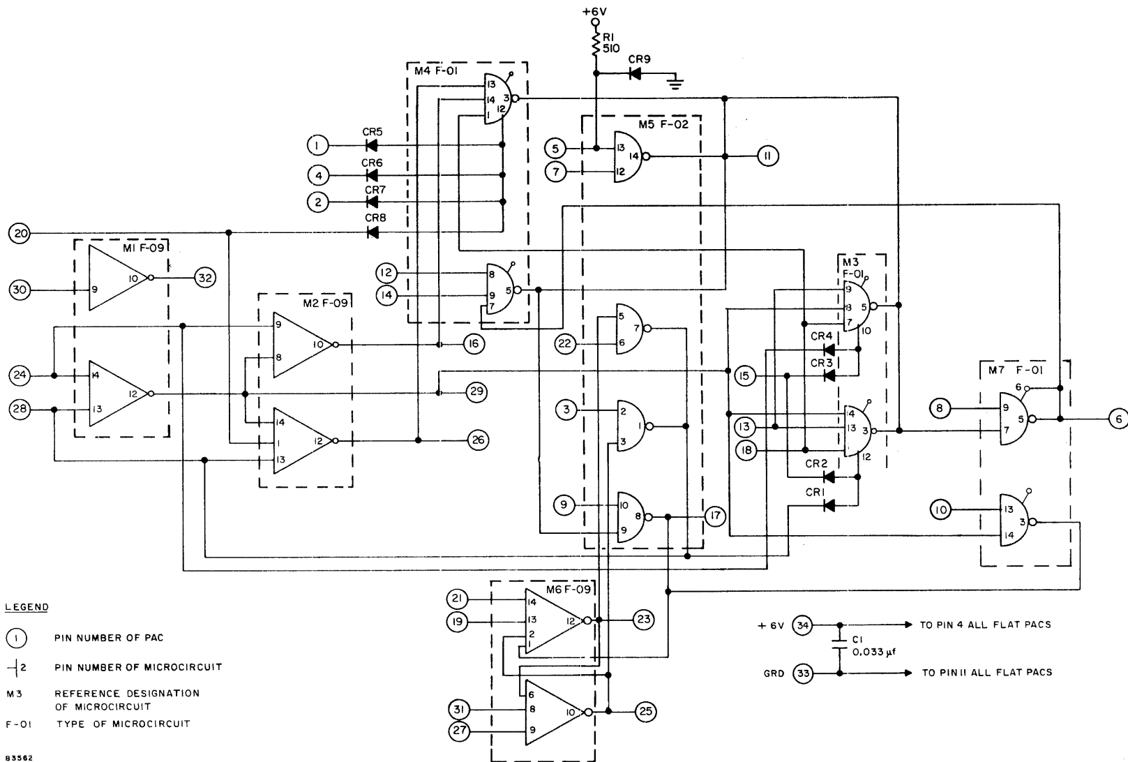
Figure A-24. Column Distribution Register and Memory Information Register Bit PAC Model CC-038
