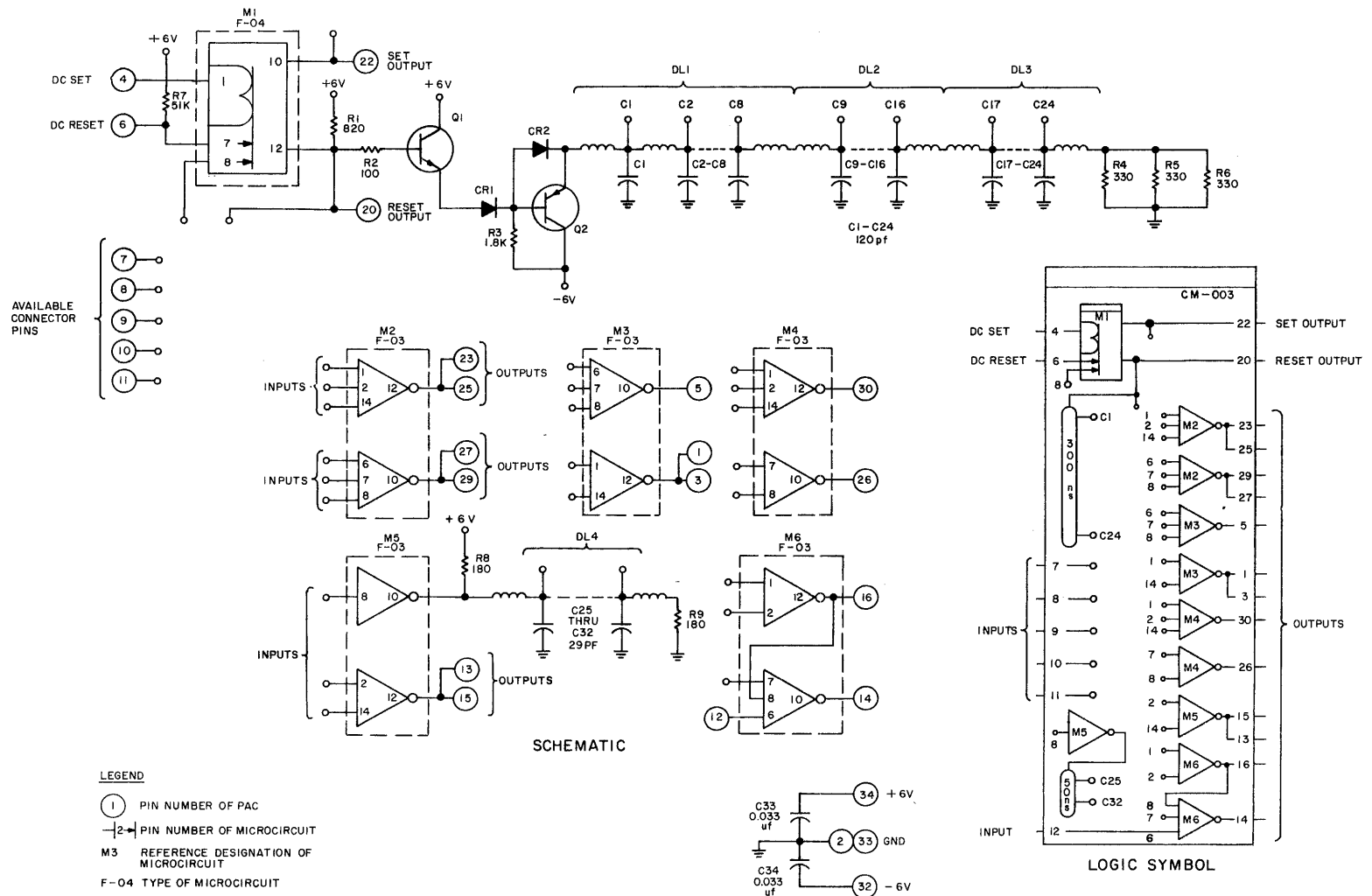
Figure A-65. Timing Distributor PAC, Model CM-003, Jumper Interconnection Diagram, Schematic Diagram, and Logic Symbol
