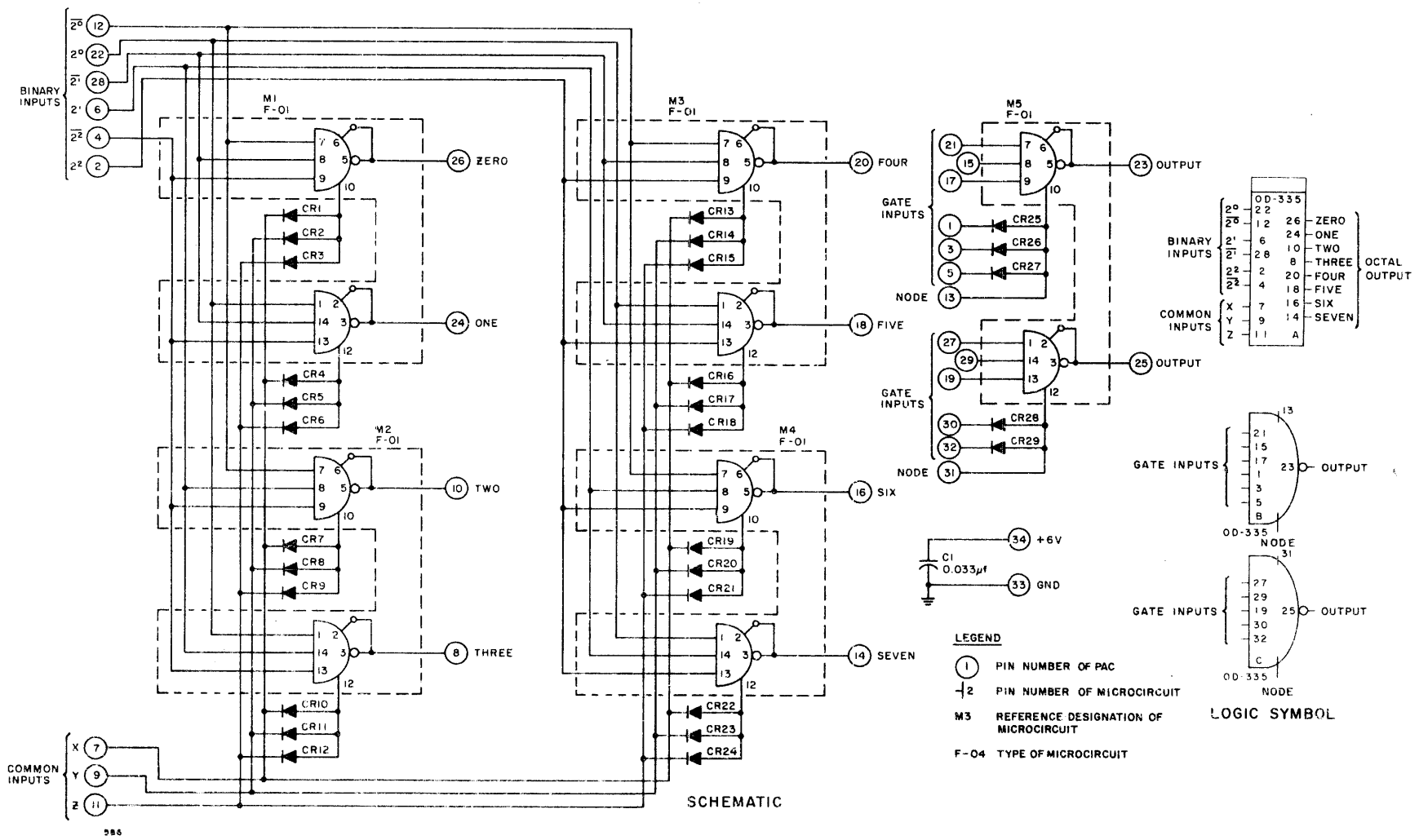
Figure A-95. Octal/Decimal Decoder PAC, Model OD-335, Schematic Diagram and Logic Symbol
