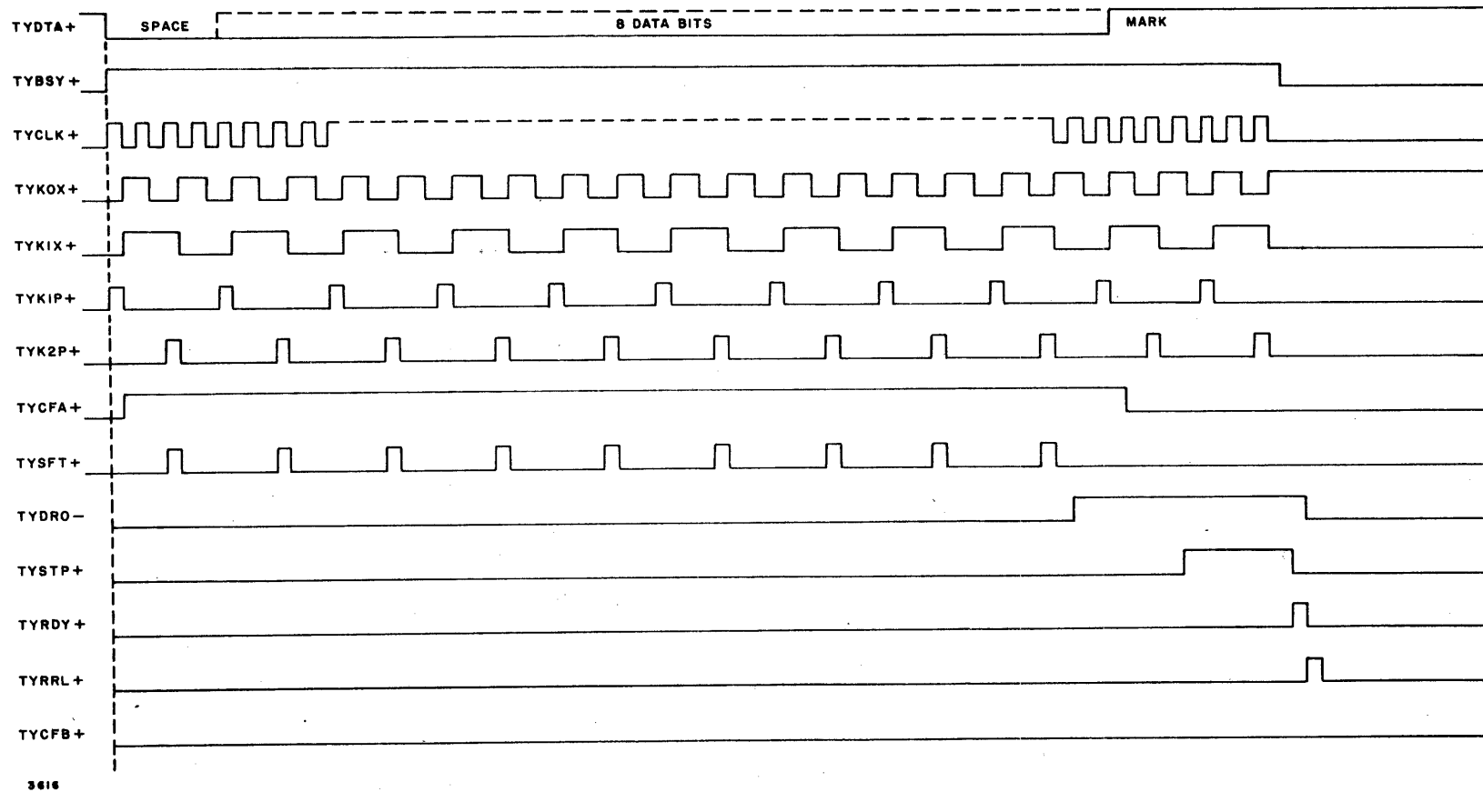
Figure 2-32. Input Mode Timing Diagram
