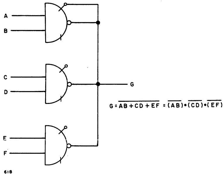
Figure A-81. NAND Type 2 PAC, Model DL-335, Gates Used in Parallel
