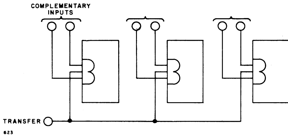
Figure A-46. Gated Flip-Flop PAC, Model CC-086, Parallel Information Drop-In
