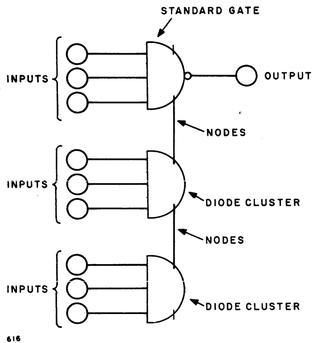
616 Figure A-75. Multi-Input NAND PAC, Model DC-335, Expansion of Gate Inputs
