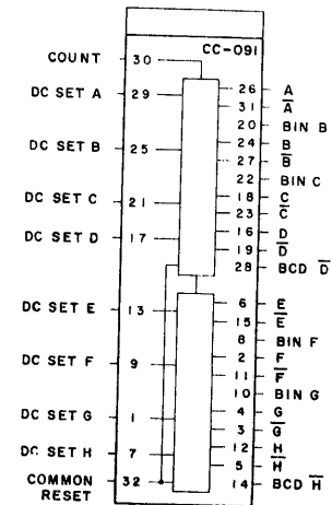
Figure A-56. Fast Carry Counter PAC, Model CC-091, Schematic Diagram and Logic Symbol
