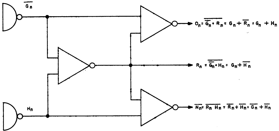
Figure 2-13. Intermediate Functions
