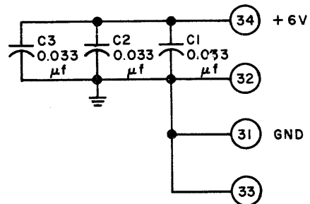
Figure A-99. Power Amplifier PAC, Model PA-335, Schematic Diagram and Logic Symbol
