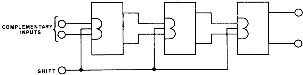
Figure A-45. Gated Flip-Flop PAC, Model CC-086, Shift Register Operation
