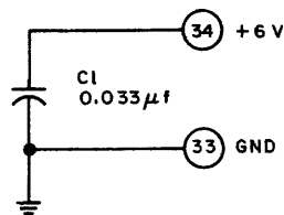
Figure A-79. NAND Type 2 PAC, Model DL-335, Schematic Diagram and Logic Symbol
