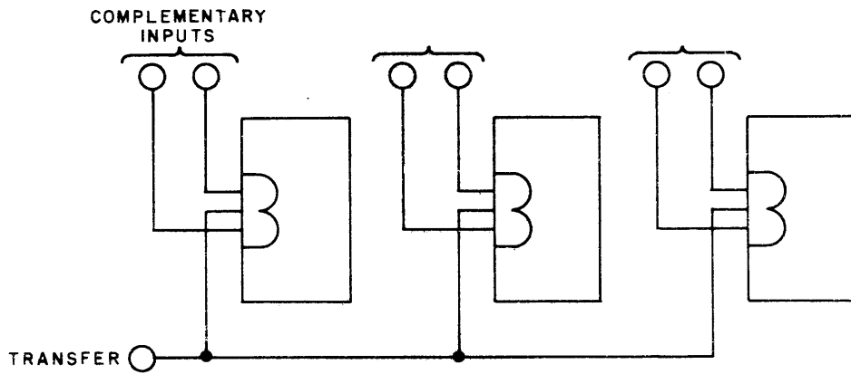
Figure A-54. Gated Flip-Flop PAC, Model CC-089, Parallel Information Drop-In
