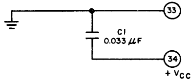
TYPICAL CIRCUIT
