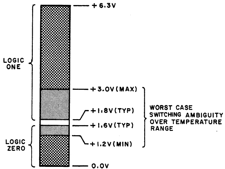
Figure A-1. Switching Thresholds
