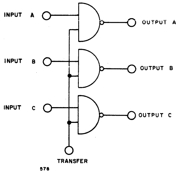
Figure A-112. Transfer Gate PAC, Model TG-335, Controlling Transfer of Three Signals
